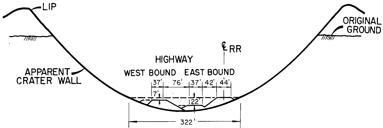
TYPICAL CROSS SECTION 50 KT CRATER SCALE: 1"=100'
